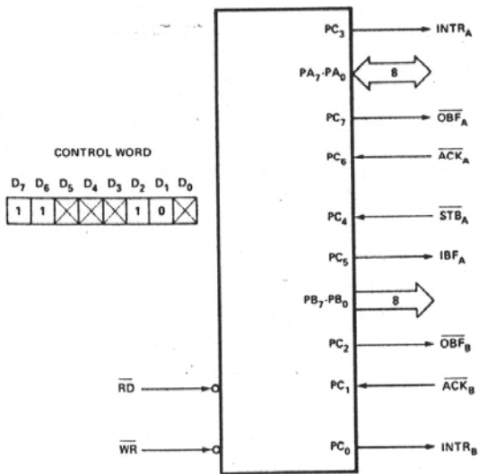
MODE 2 AND MODE 1 (OUTPUT)
