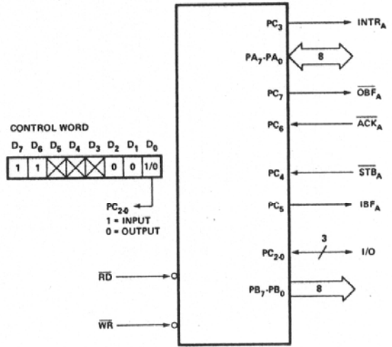
MODE 2 AND MODE 0 (OUTPUT)
