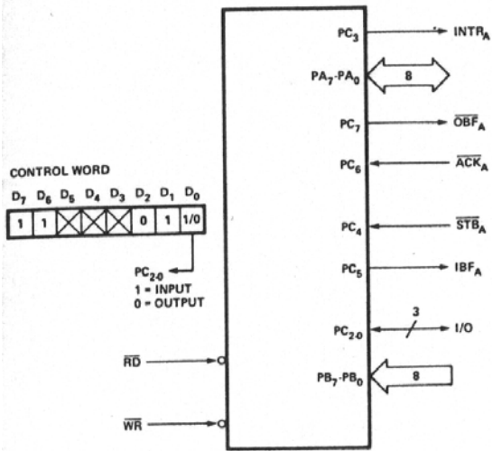
MODE 2 AND MODE 0 (INPUT)
