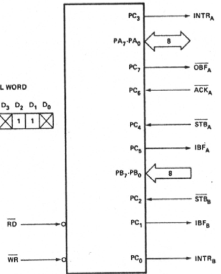
MODE 2 AND MODE 1 (INPUT)
