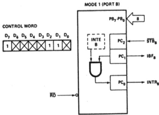
PORT A, B — (STROBED INPUT)
