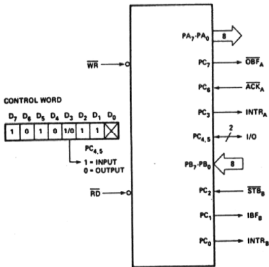
PORT A — (STROBED OUTPUT) PORT B — (STROBED INPUT)
