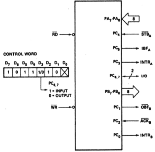
PORT A — (STROBED INPUT) PORT B — (STROBED OUTPUT)
